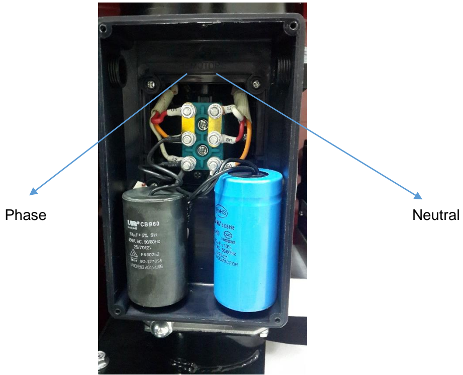
Photo 7. Connection on 220 V AC mono phase motors*
