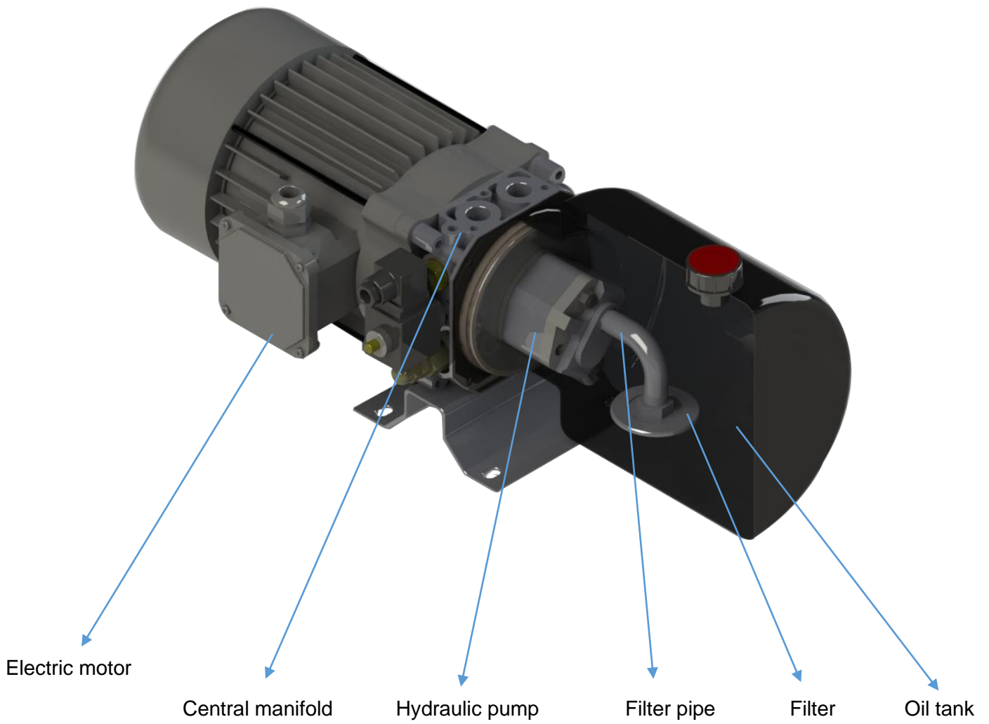
Photo 2. Main components of mini power pack
