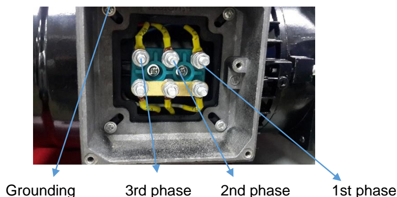
Photo 6. Connection on 380 V AC three phase motors
