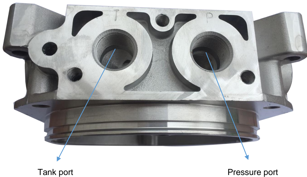
Photo 5. Connection ports on central manifold
