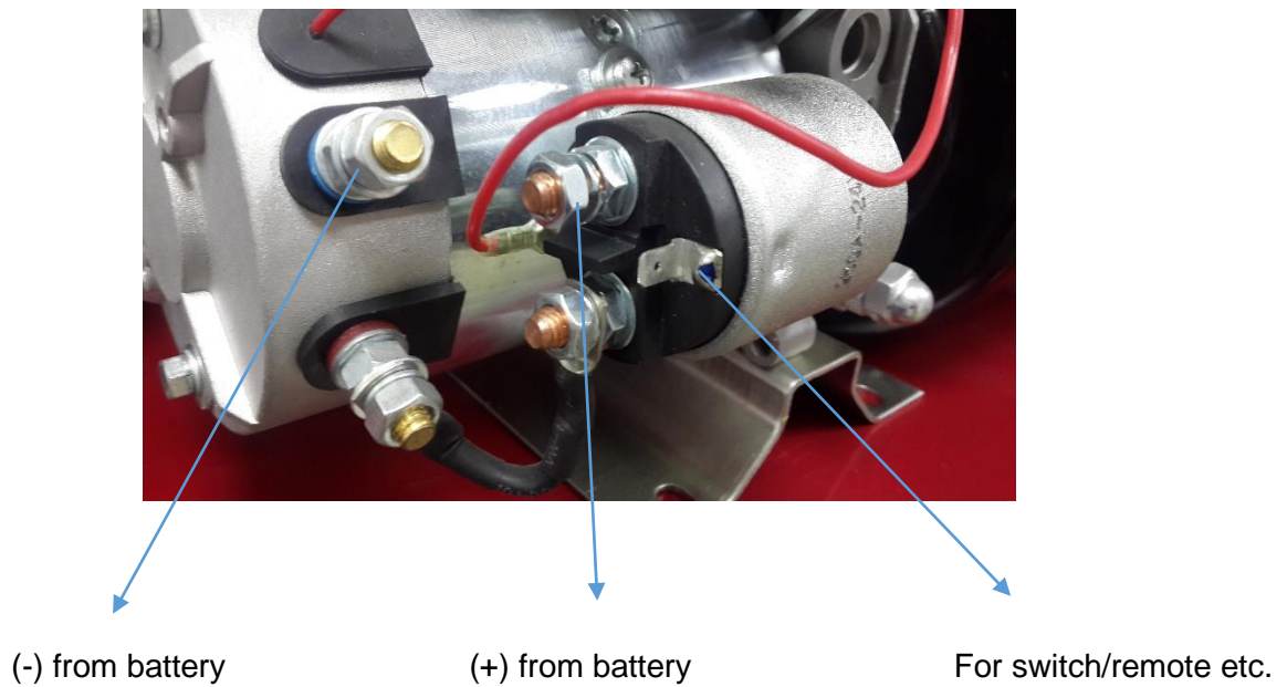
Photo 8. Connection on DC motor
