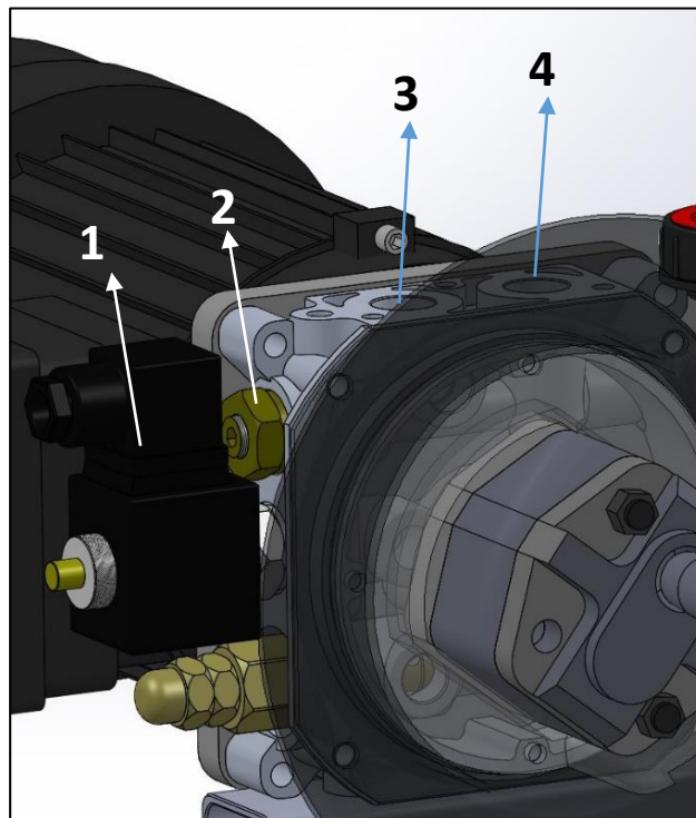
Photo 3. Single acting power unit
