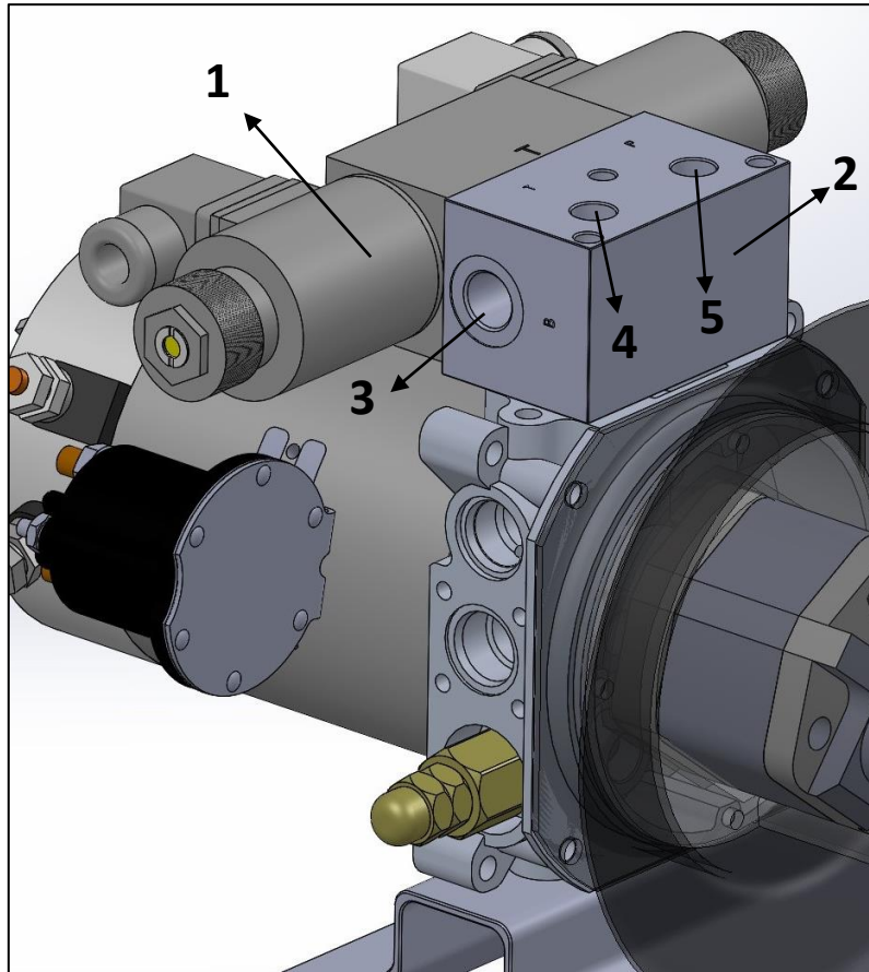
Photo 4. Double acting power unit
